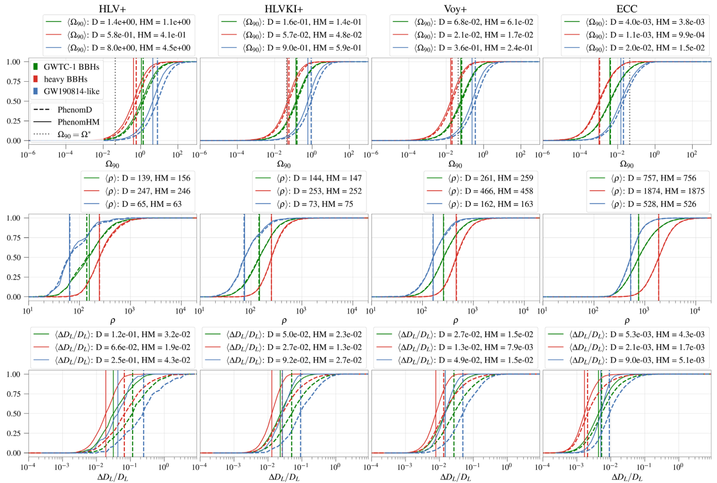
Figure 3. Cumulative density functions and medians of the 90% credible sky area \Omega_{90} , S/N \rho , and fractional luminosity distance error \Delta D_L / D_L calculated with two waveform models, one including higher modes (PhenomHM, solid) and the other without (PhenomD, dashed), for the GWTC-1 BBH, heavy BBH, and GW190814-like populations. S/Ns and distance errors are restricted to systems fulfilling \Omega_{90} < \Omega^* .
