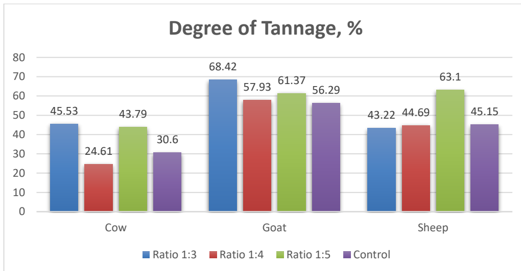
Fig. 2. Degree of tannage for various feeding ratio on cow, goat, and sheep leather
