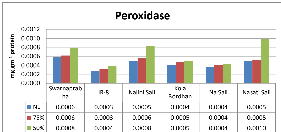
Fig. 3. Effect of low light on Peroxidase activity
