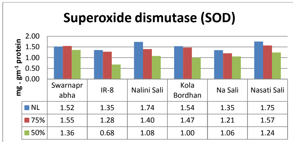
Fig. 1. Effect of low light on Superoxide dismutase (SOD) activity
