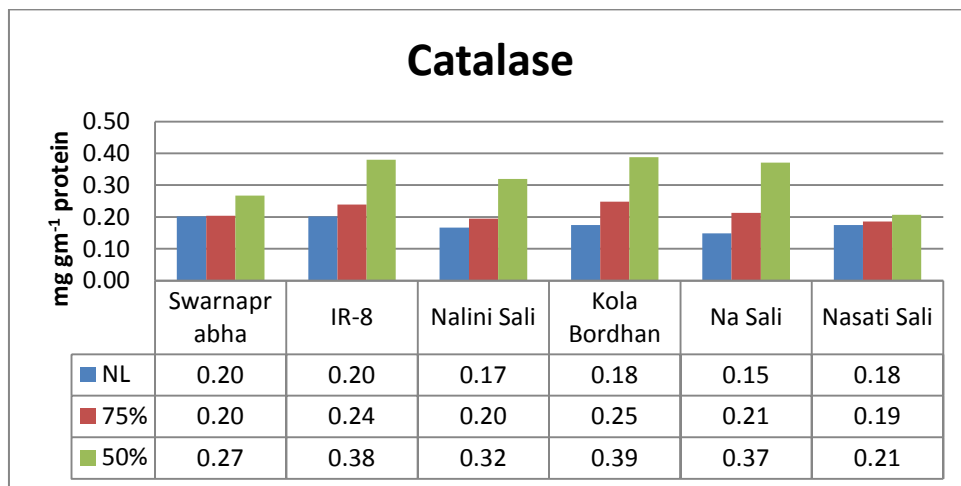
Fig. 2. Effect of low light on Catalase activity
