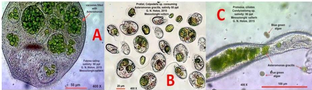
Fig. 4. Ciliated protozoa fed to satiation with A. gracilis cells. A - Fabrea salina . B - Colpodella sp. C - Condylostoma sp.
