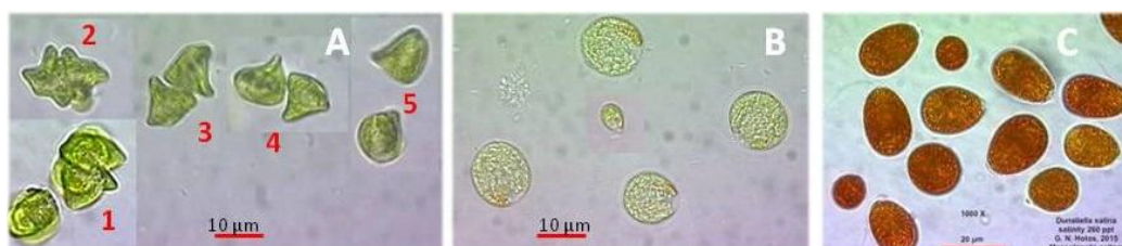
Fig. 3. A- (1-5) advancement of cell division stages in A. gracilis . B- Swollen spherical cells of A. gracilis full of vesicles after lowering salinity, a faint orange colored eye spot can be seen, in the center of the picture a cell of Dunaliella can be seen for the sake of size comparisons. C- Typical pear-shaped cells of Dunaliella salina full of carotenoids
