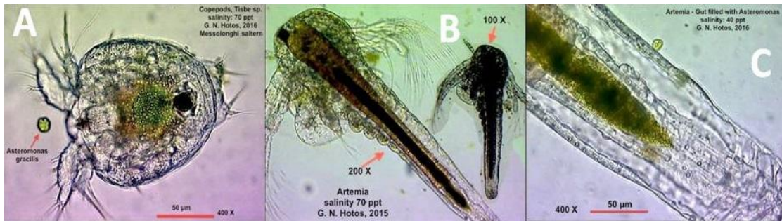
Fig. 6. A - Copepod Tisbe sp. nauplius fed to satiation with A. gracilis . B - Artemia sp. with its alimentary canal full of A. gracilis . C - Close view of the Artemia 's alimentary canal full of A. gracilis cells
