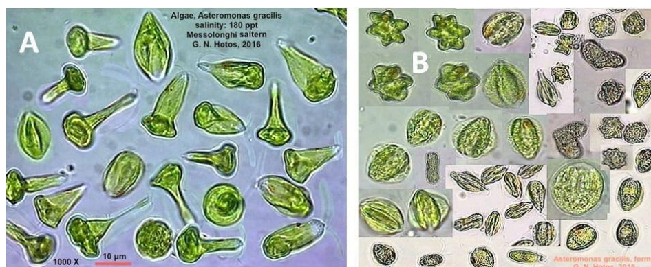
Fig. 2. A - A. gracilis in nail-like form in very high salinity (180 ppt). B - A collage of A. gracilis various forms
