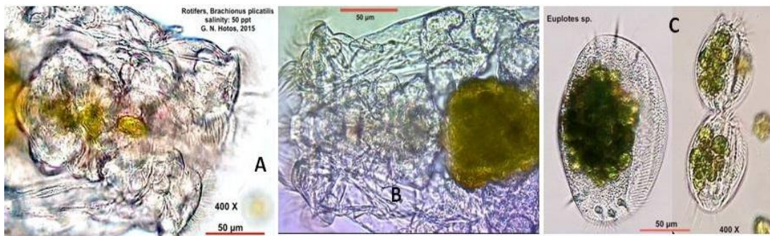
Fig. 5. A - Rotifer B. plicatilis just “swallowing” a A. gracilis cell while many more are smashed in its mastax. B - Gut of B. plicatilis full with A. gracilis cells in digestion. C - Protozoa, Euplotes sp. fed to satiation with A. gracilis
