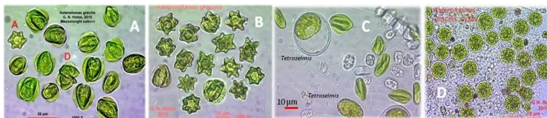
Fig. 1. A - Asteromonas gracilis in its most usual form (A: indicates a stellate appearance, D: cell division). B- Stellate-shaped cells. C- Cells of A. gracilis among salt crystals, there also depicted 2 cells of Tetraselmis marina one in palmelloid stage and one vegetative in order to compare sizes. D - Cysts of A. gracilis
