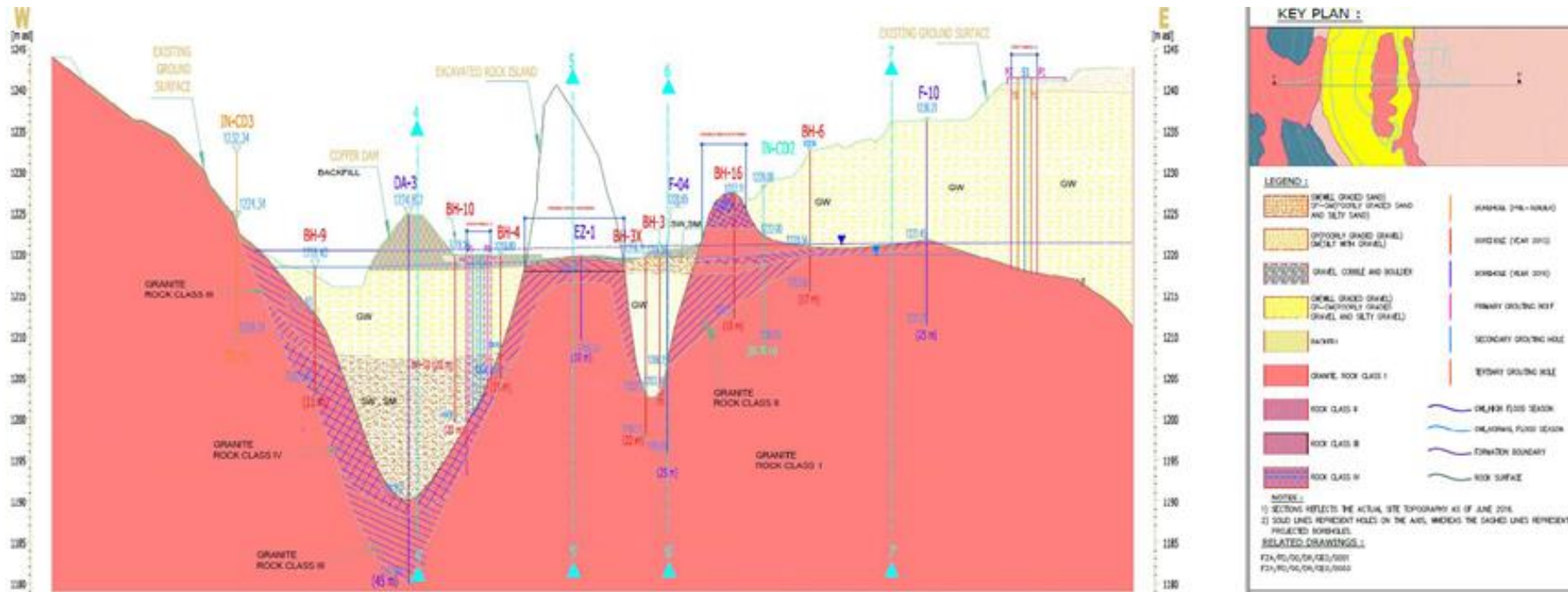
Fig. 5. Engineering geological cross section at dam axis [11]
