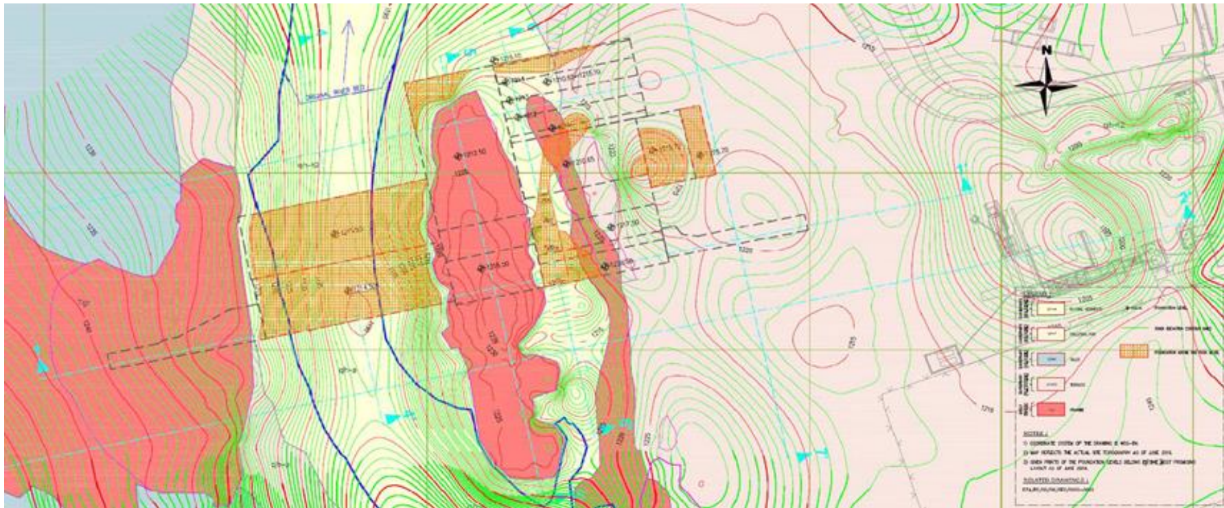
Fig. 4. Detailed geological engineering map indicating plant foundation area [12]
