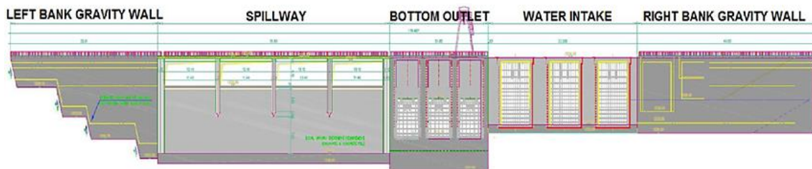
Fig. 2. Diagram showing the cross-section on the dam axis [12]
