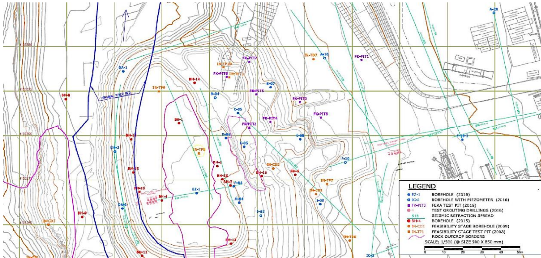
Fig. 3. Boreholes locations of hydropower plant project [12]
