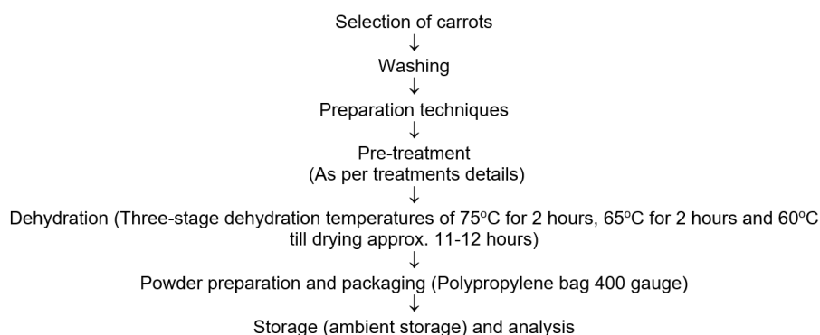
Fig. 1. Principal steps used for dehydration of carrot into powder
