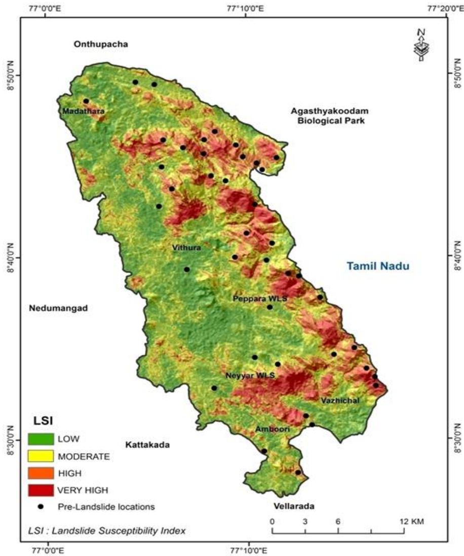
Fig. 4. Landslide susceptibility index map
