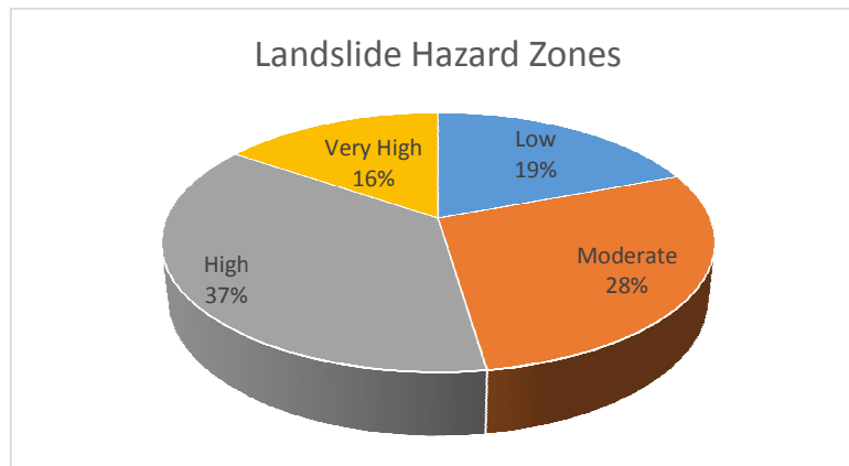
Fig. 5 Landslide hazard zones
