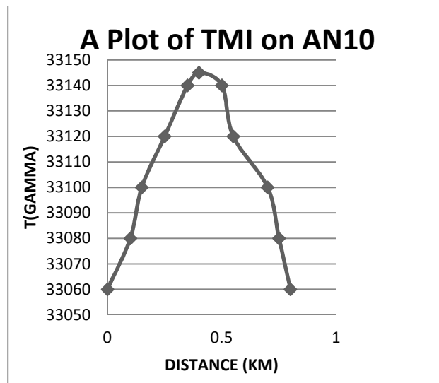
Fig. 5.4. Magnetic intensity against distance of anomaly 10
