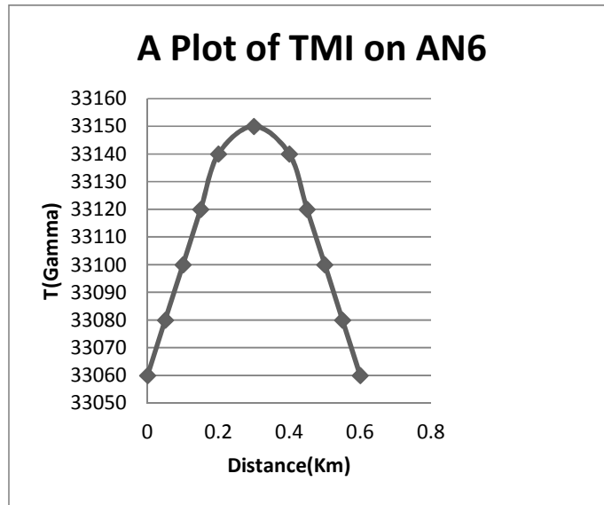
Fig. 5.3. Magnetic intensity against distance of anomaly 6
