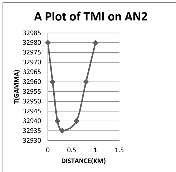
Fig. 5.2. Magnetic intensity against distance of anomaly 2
