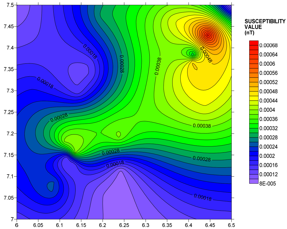
Fig. 3. Magnetic susceptibility map of the study area showing rock contrasts
