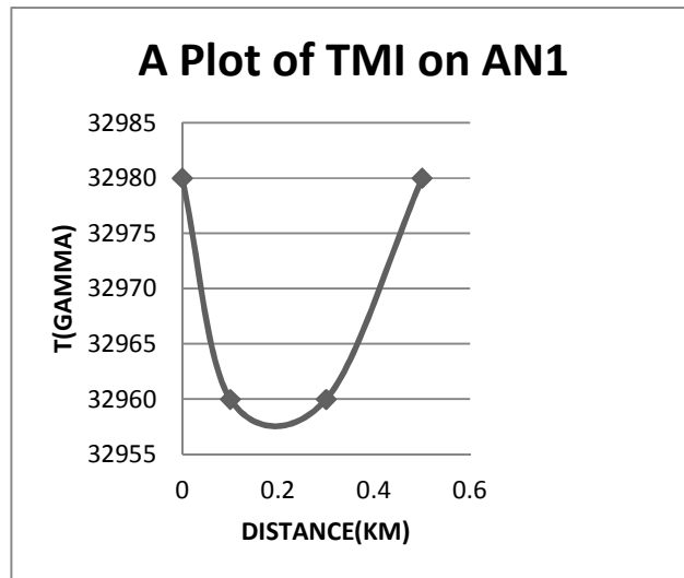
Fig. 5.1. Magnetic intensity against distance of anomaly 1
