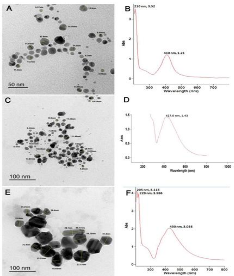
Fig. 1. Shape, size and surface plasmon resonance peaks (SPR) of Ag-NPs by TEM and UV-Vis (A) Shape and size of PVP-Ag-NPs by TEM. (B) SPR of PVP-Ag-NPs by UV-Vis. (C) Shape and size of PVP-Glu-Ag-NPs by TEM. (D) SPR of PVP-Glu-Ag-NPs by UV-Vis. (E) Shape and size of Cit-Ag-NPs by TEM. (F) SPR of Cit-Ag-NPs by UV-Vis
