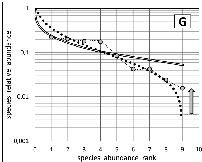
Fig. 15. The new Species Abundance Distribution when community “G” has reached stage 2 ( S_t = 9 ; I_{str} = 0.83 ) as a consequence of the environmental peioration (see Fig. 14). The arrow highlights the beginning separation from the log-normal model (dotted line) towards the “log-series” model (double line). Initial situation (step 0) of community “G” is provided at Fig. 2
